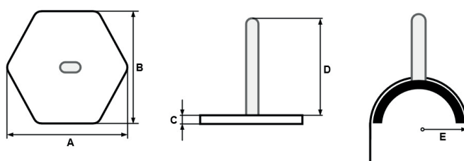
LOOP® Flexi Stickon glued to the curved surface of a boom
